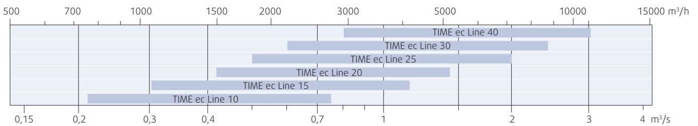
Airflow for TIME ec Line with external pressure of 250 Pa and max SFP 2.1 kW/(m 3 /s).
